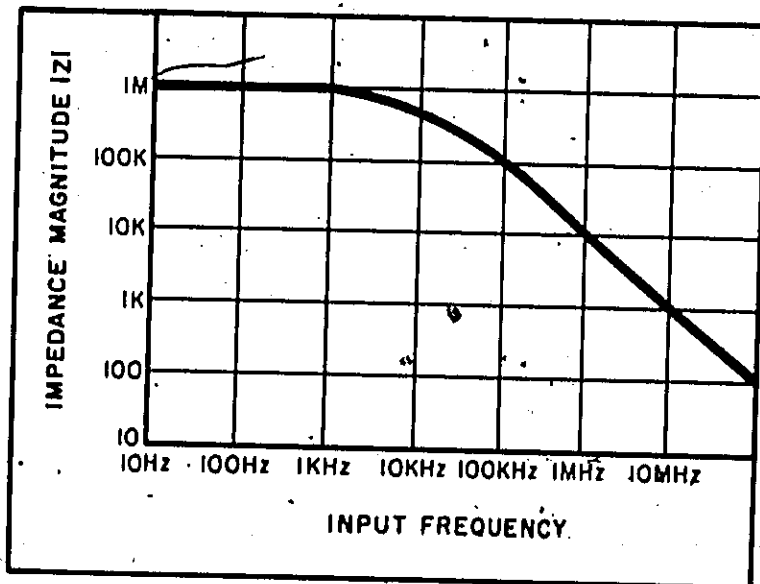
Figure 3-21. Model 5261A Input Impedance.
